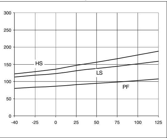
Figure 8. Propagation delays [ns] low to high vs. T_J
