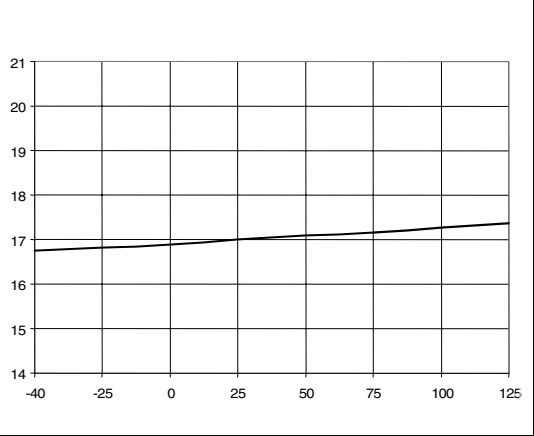
Figure 6. Overcurrent protection threshold [V] vs. T_J
