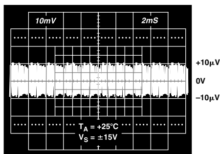
TPC 17. Low Frequency Voltage Noise
