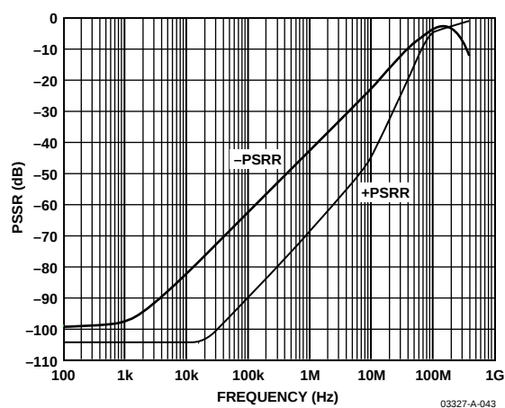
Figure 44. PSRR vs. Frequency
