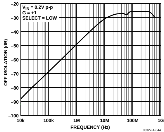
Figure 45. Off Isolation vs. Frequency
