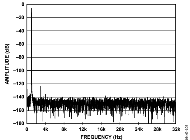
Figure 11. AD7766-1 FFT, 1 kHz, -6 dB Input Tone
