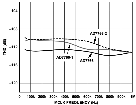
Figure 19. AD7766/AD7766-1/AD7766-2 THD vs. MCLK Frequency
