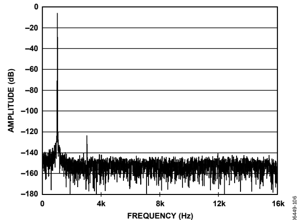
Figure 12. AD7766-2 FFT, 1 kHz, -6 dB Input Tone
