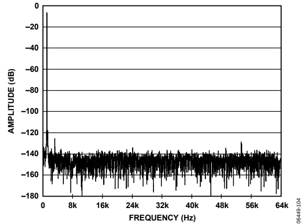
Figure 10. AD7766 FFT, 1 kHz, -6 dB Input Tone
