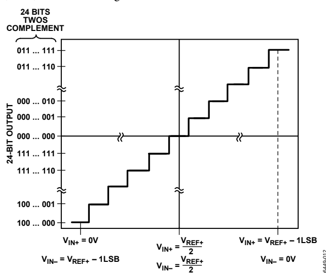
Figure 28. AD7766/AD7766-1/AD7766-2 Transfer Function
