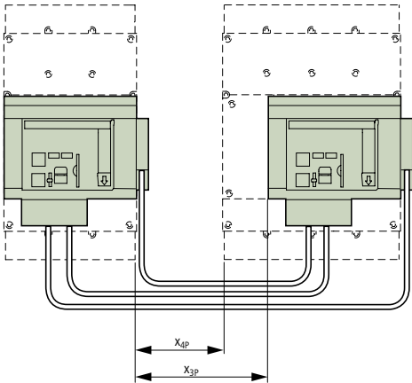
Mechanical interlock, XMVR (mounting side-by-side)
