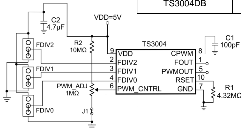
Figure 1. TS3004 Demo Board Circuit
