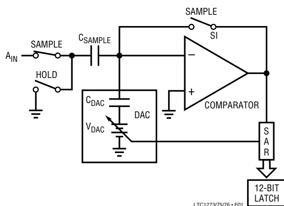
Figure 1. A_{IN} Input
