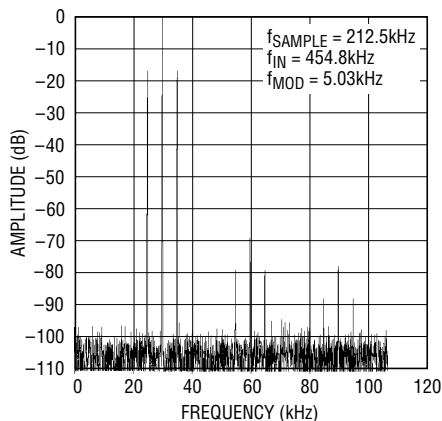
Figure 24. 455kHz Input Voltage Modulated by a 5kHz Signal
