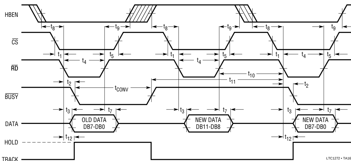
Figure 16. ROM Mode Two Byte Read Timing Diagram
