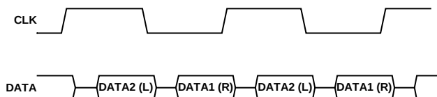
Figure 10. Stereo PDM Format
