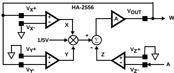
FIGURE 5. SQUARE ROOT (FOR A &gt; 0)
