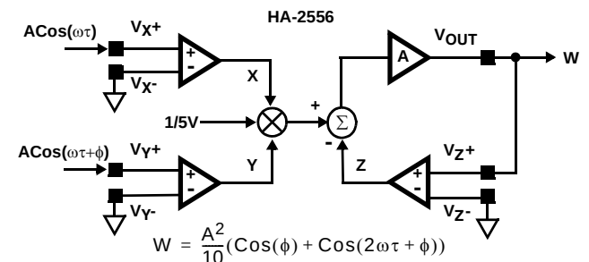
FIGURE 8. PHASE DETECTION
