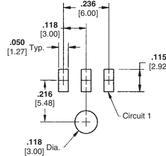
Recommended PC Board Layout * 3 Position
