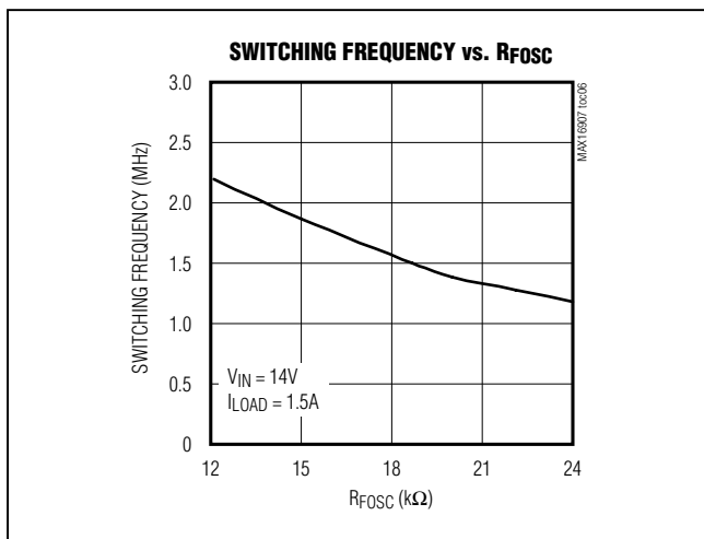
Figure 2. Switching Frequency vs. R_{\text{FOSC}}
