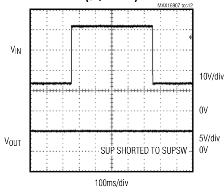
LOAD DUMP TEST (5V/2.2MHz)
