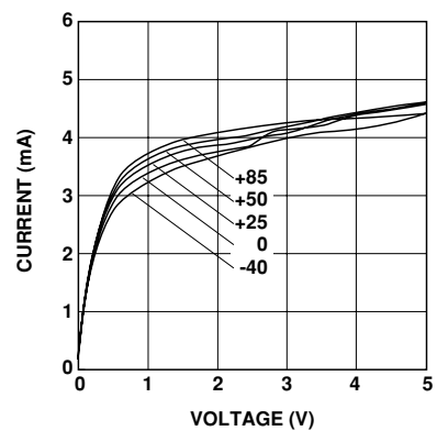
Figure 9. Device Current vs. Voltage.
