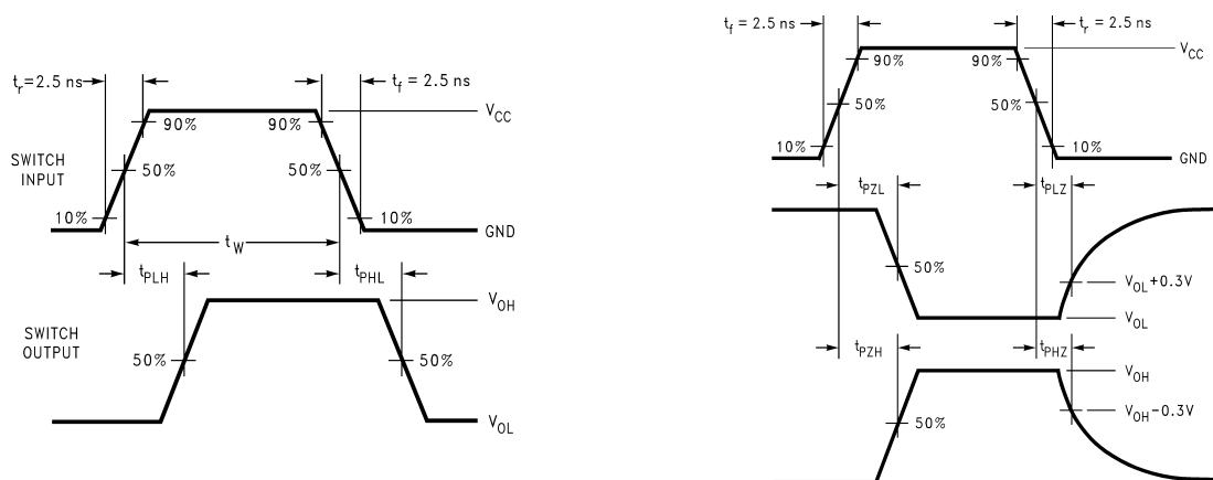
FIGURE 2. AC Waveforms
