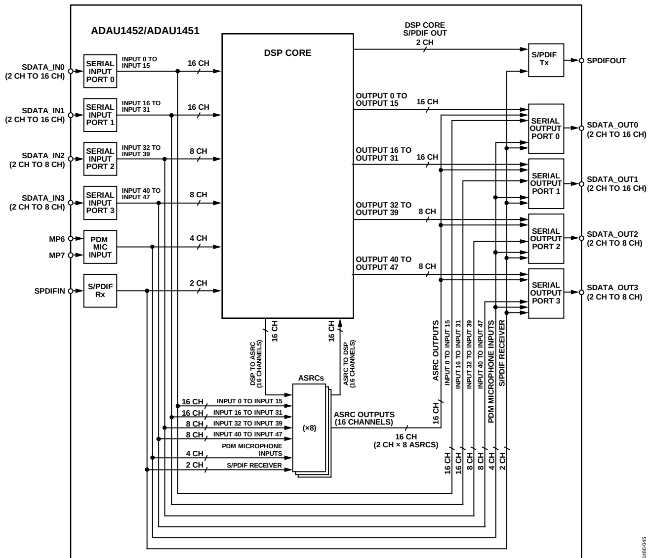
Figure 42. Audio Routing Overview
