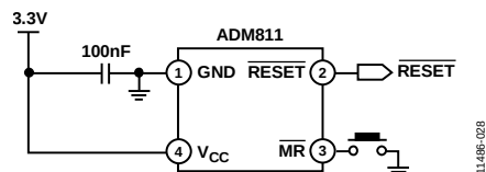
Figure 24. Example Manual Reset Generation Circuit
