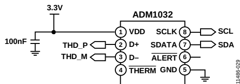
Figure 26. Example External Temperature Sensor Circuit
