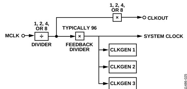
Figure 21. Clock Output Generator
