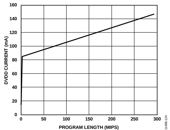
Figure 25. ADAU1452 Typical DVDD Current Draw vs. Program MIPS at an Ambient Temperature of 25°C and a Sample Rate of 48 kHz
