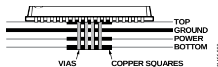
Figure 84. Exposed Pad Layout Example—Side View
