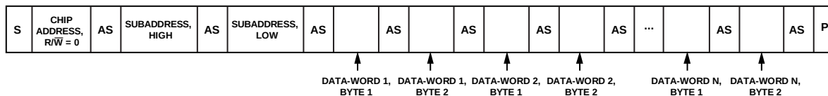
Figure 31. Simplified Burst Mode I 2 C Write Sequence
