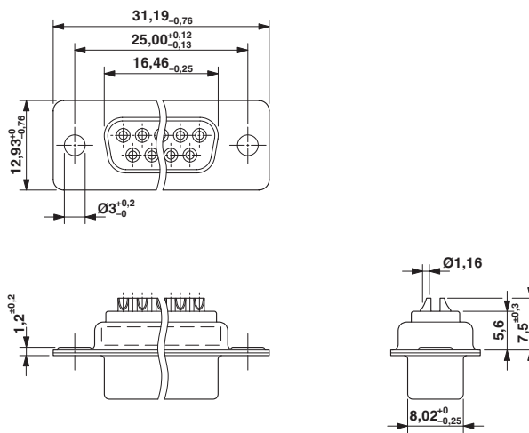
D-SUB contact insert
