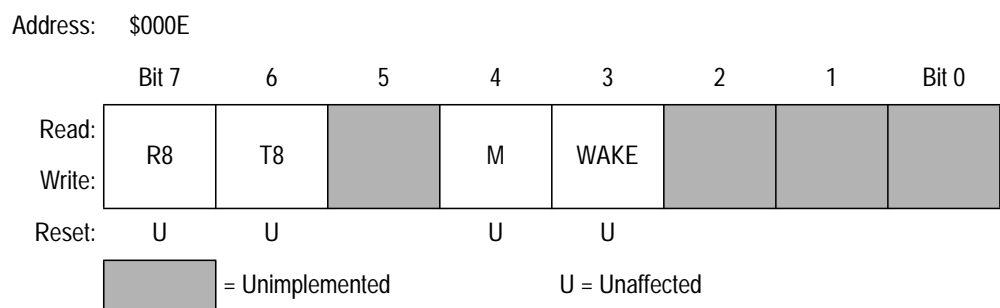
Figure 10-6. SCI Control Register 1 (SCCR1)
