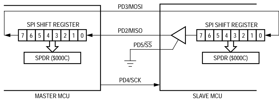
Figure 11-3. Master/Slave Connections
