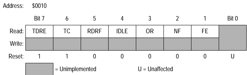
Figure 10-8. SCI Status Register (SCSR)
