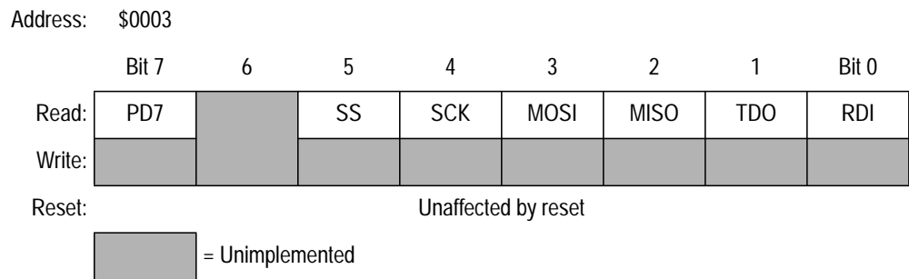
Figure 7-10. Port D Fixed Input Register (PORTD)
