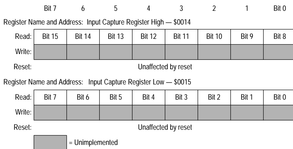
Figure 8-11. Input Capture Registers (ICRH and ICRL)
