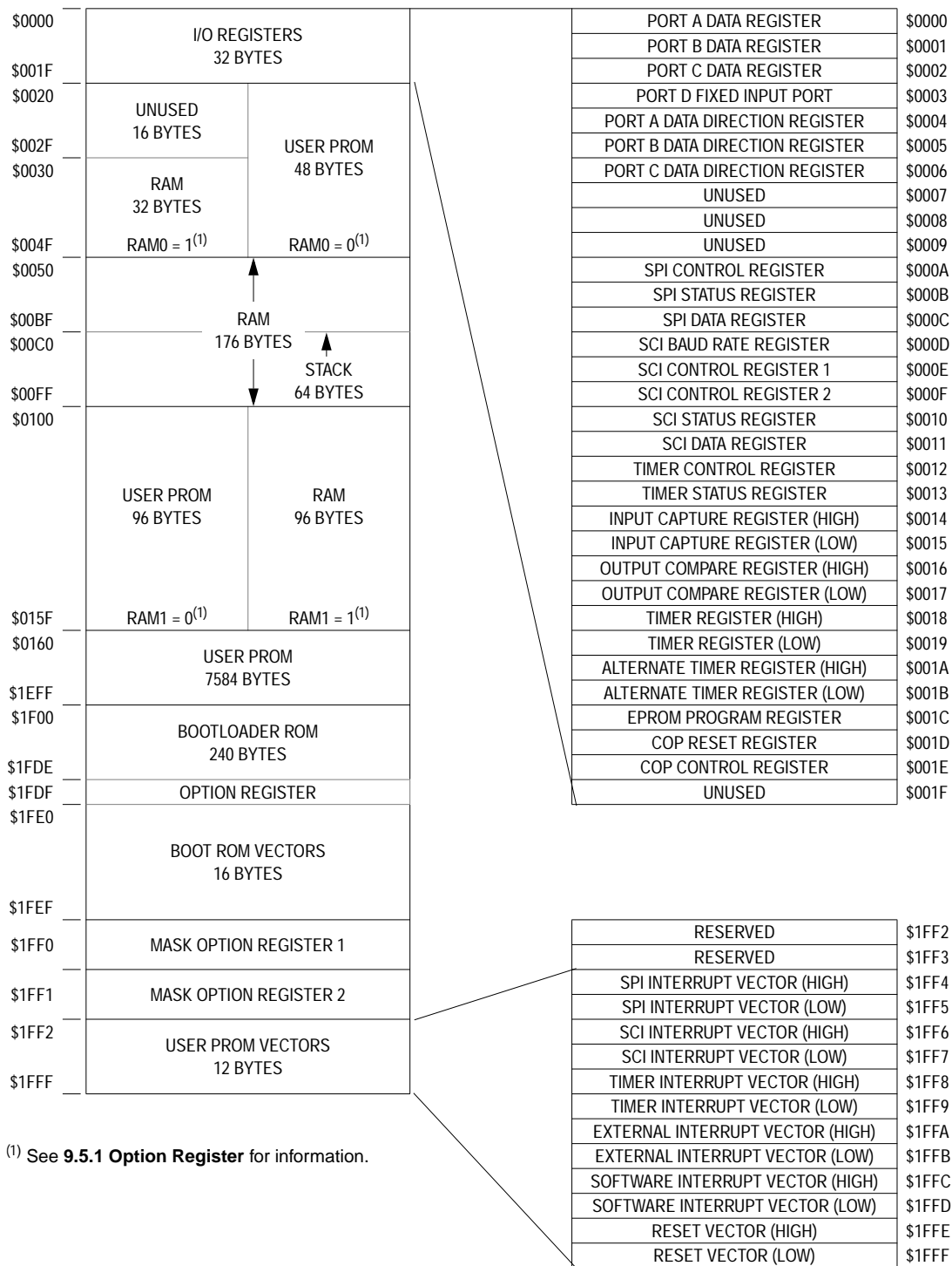
Figure 2-1. Memory Map
