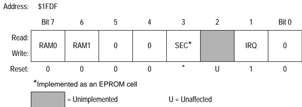
Figure 1-1. Option Register (Option)
