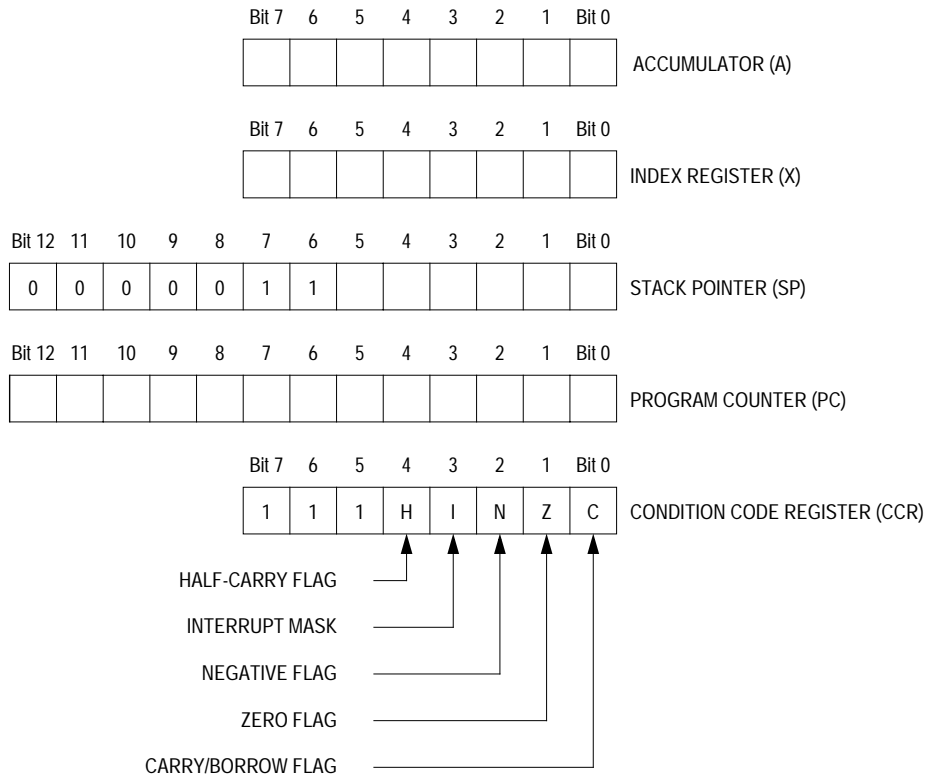
Figure 3-1. Programming Model
