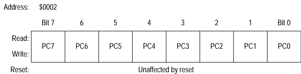
Figure 7-7. Port C Data Register (PORTC)
