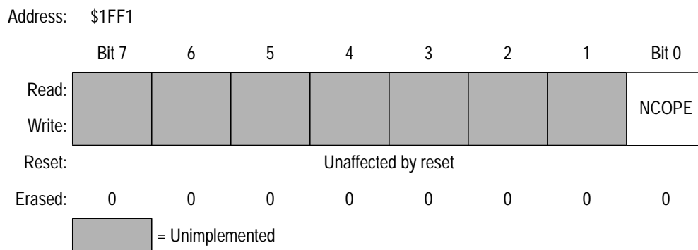
Figure 9-6. Mask Option Register 2 (MOR2)
