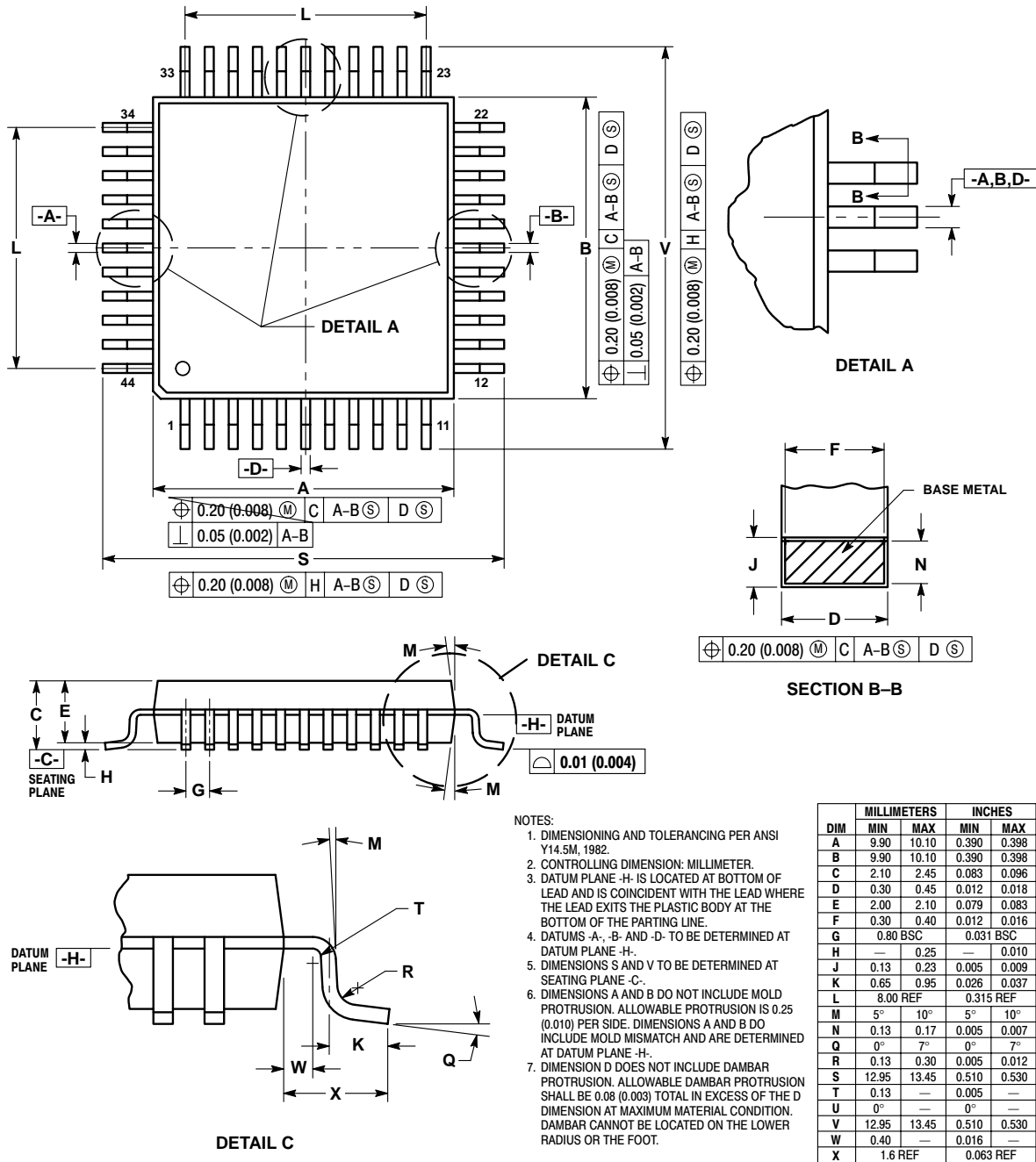
Figure 14-5. MC68HC705C8AFB Package Dimensions (Case #824E)
