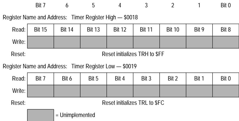
Figure 8-7. Timer Registers (TRH and TRL)
