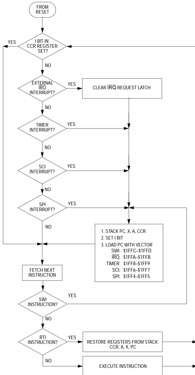
Figure 4-5. Reset and Interrupt Processing Flowchart
