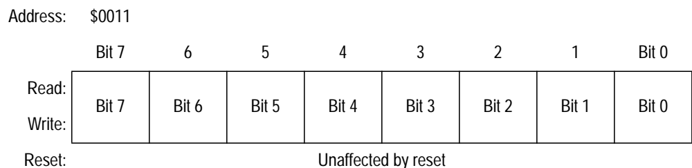
Figure 10-5. SCI Data Register (SCDR)
