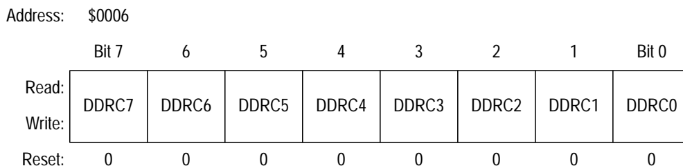
Figure 7-8. Data Direction Register C (DDRC)
