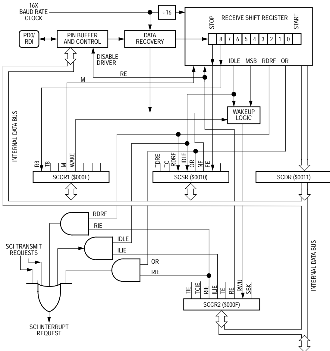
Figure 10-4. SCI Receiver
