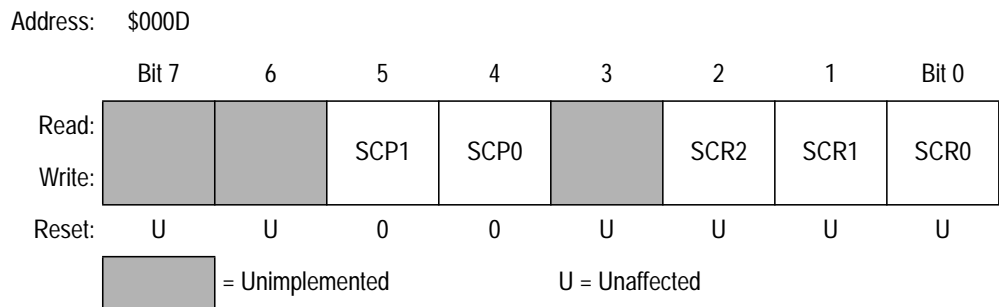
Figure 10-9. Baud Rate Register (Baud)
