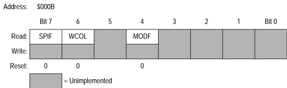
Figure 11-9. SPI Status Register (SPSR)
