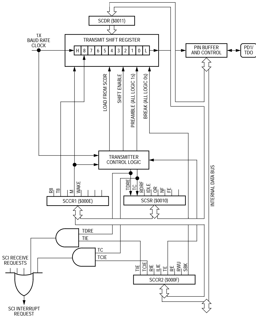
Figure 10-2. SCI Transmitter
