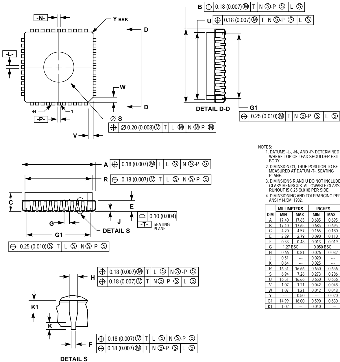
Figure 14-4. MC68HC705C8AFS Package Dimensions (Case #777B)
