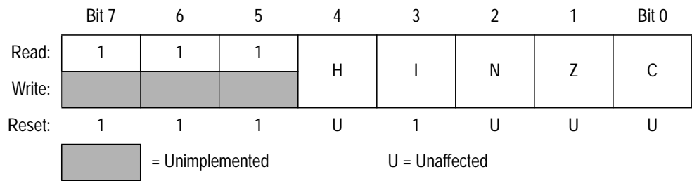
Figure 3-6. Condition Code Register (CCR)
