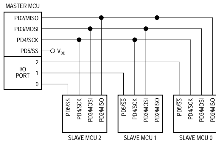
Figure 11-4. One Master and Three Slaves Block Diagram
