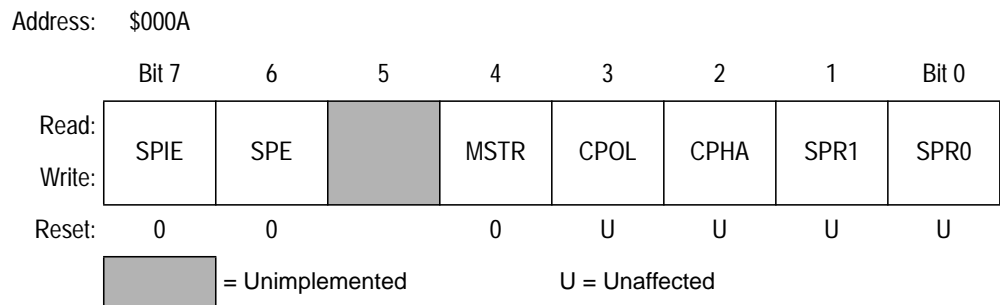
Figure 11-8. SPI Control Register (SPCR)
