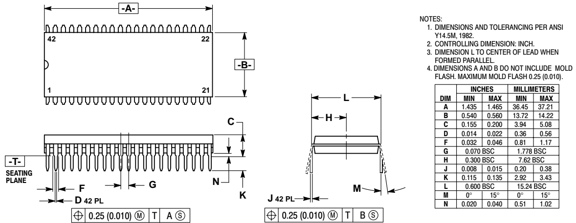
Figure 14-6. MC68HC705C8AB Package Dimensions (Case #858)
