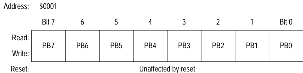
Figure 7-4. Port B Data Register (PORTB)
