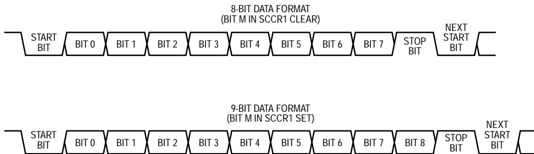
Figure 10-1. SCI Data Format
