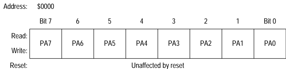
Figure 7-1. Port A Data Register (PORTA)
