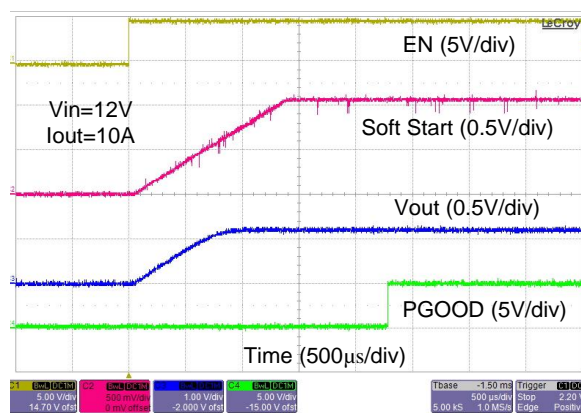
Figure 12. Startup Waveforms with 10 A Load Current
