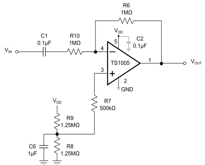
Figure 4. Inverting Configuration
