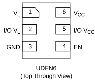
Figure 2. Pinout Diagram
