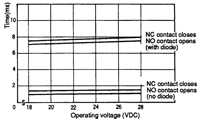
Example of Operating Voltage to Reset Time
