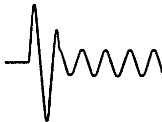
Current Waveform when Solenoid is Switched ON
