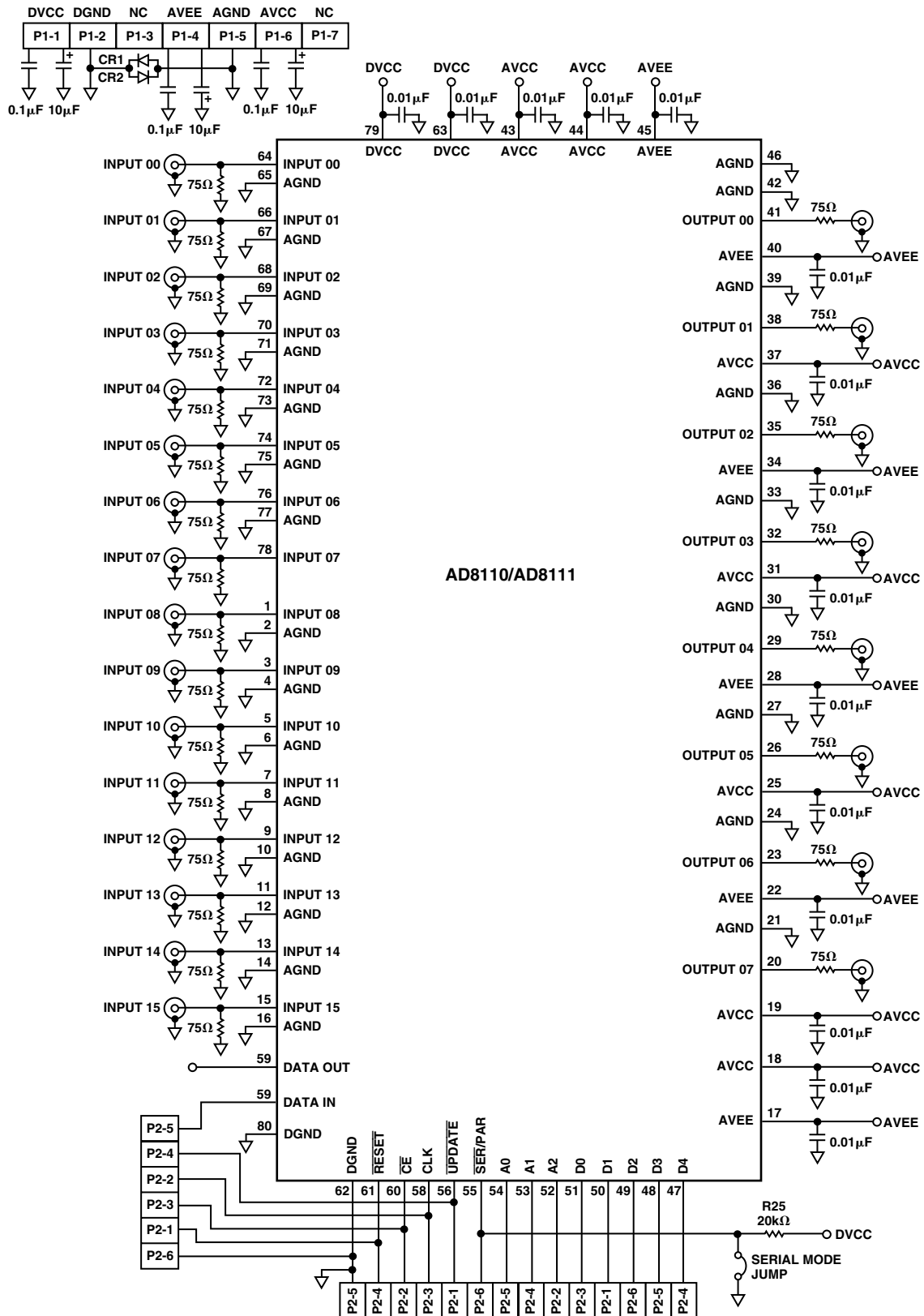
Figure 9. Evaluation Board Schematic
