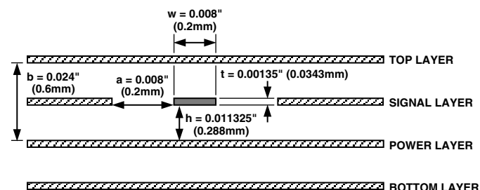
Figure 8. Cross Section of Input and Output Traces
