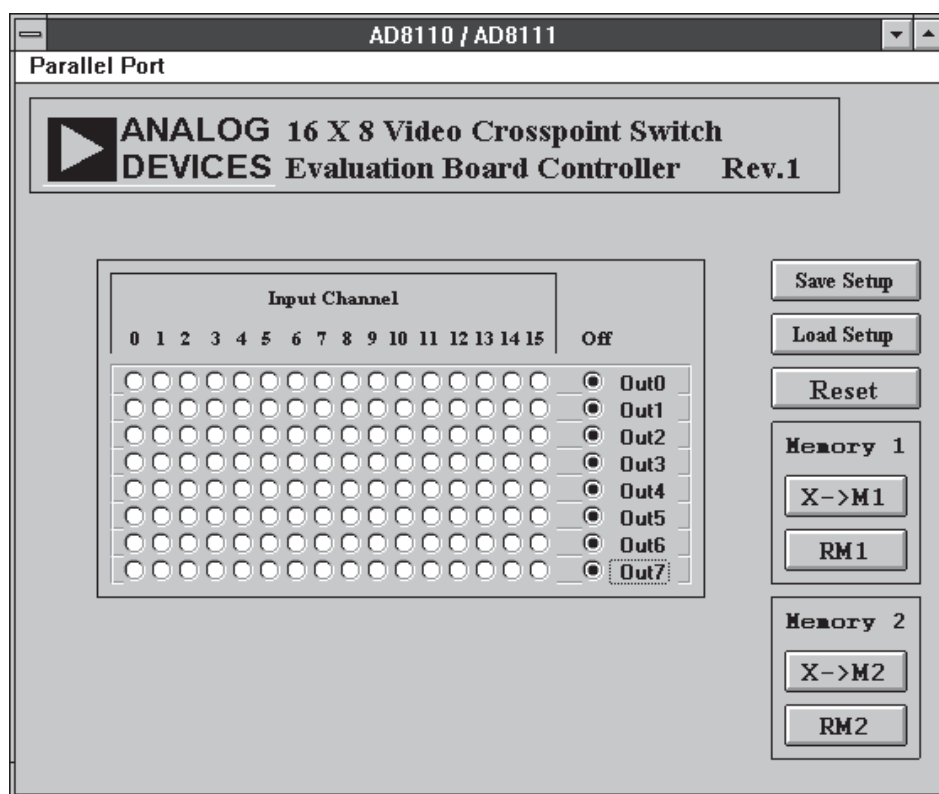
Figure 16. Evaluation Board Control Panel
