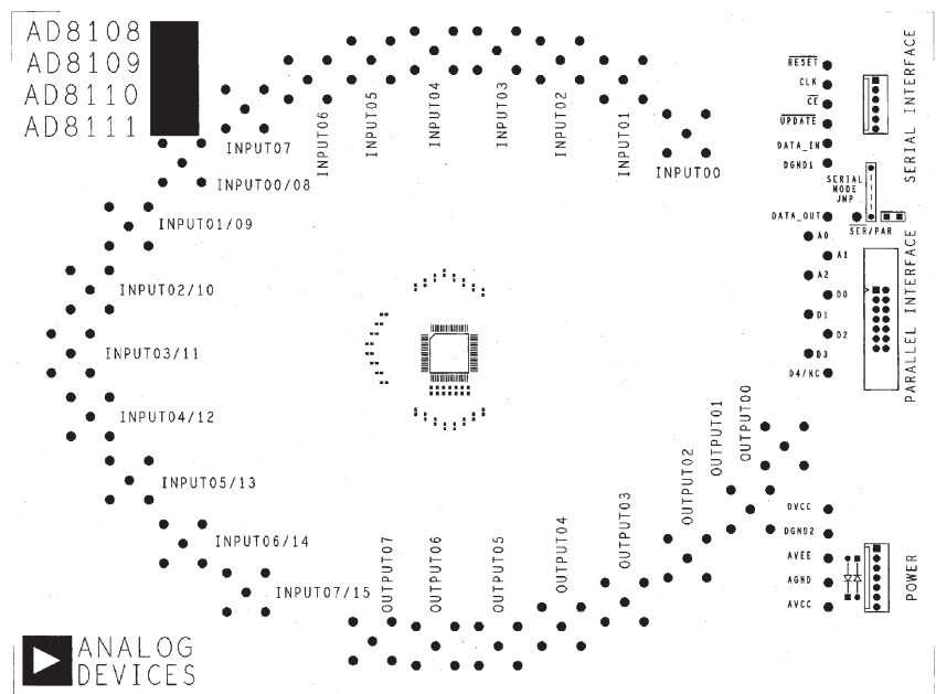
Figure 10. Component Side Silkscreen
