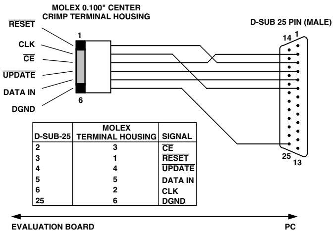
Figure 15. Evaluation Board-PC Connection Cable
