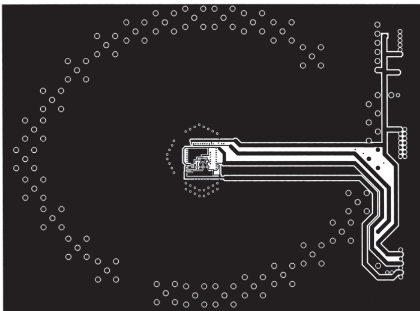
Figure 13. Board Layout (Power Plane)
