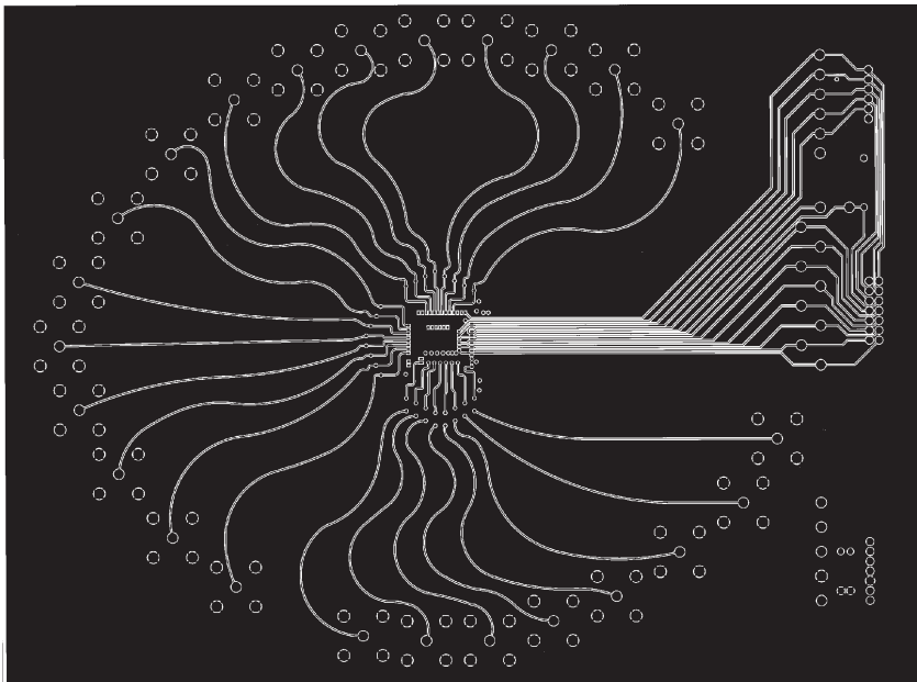
Figure 12. Board Layout (Signal Layer)
