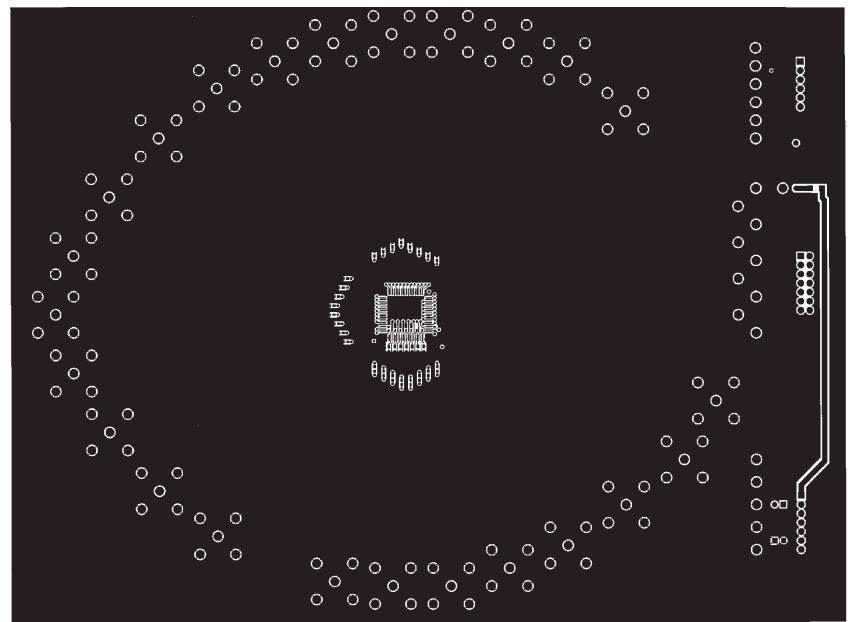
Figure 11. Board Layout (Component Side)
