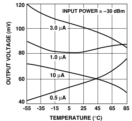
Figure 25. Output Voltage vs. Temperature and Bias Current in the 915 MHz Voltage Doubler using the HSMS-286C.
