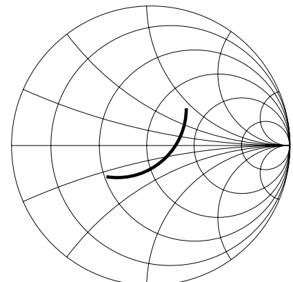
FREQUENCY (GHz): 5.6-6.0
