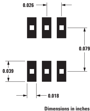
Figure 34. Recommended PCB Pad Layout for Avago's SC70 6L/SOT-363 Products.
