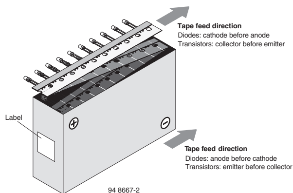
Fig. 22 - Tape Direction
