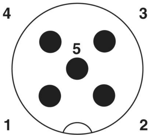
Schematic diagram
