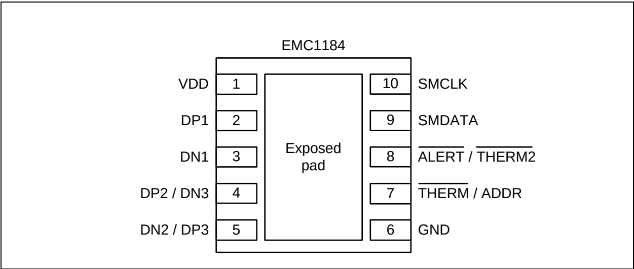
Figure 2.1 EMC1184 Pin Diagram DFN-10
