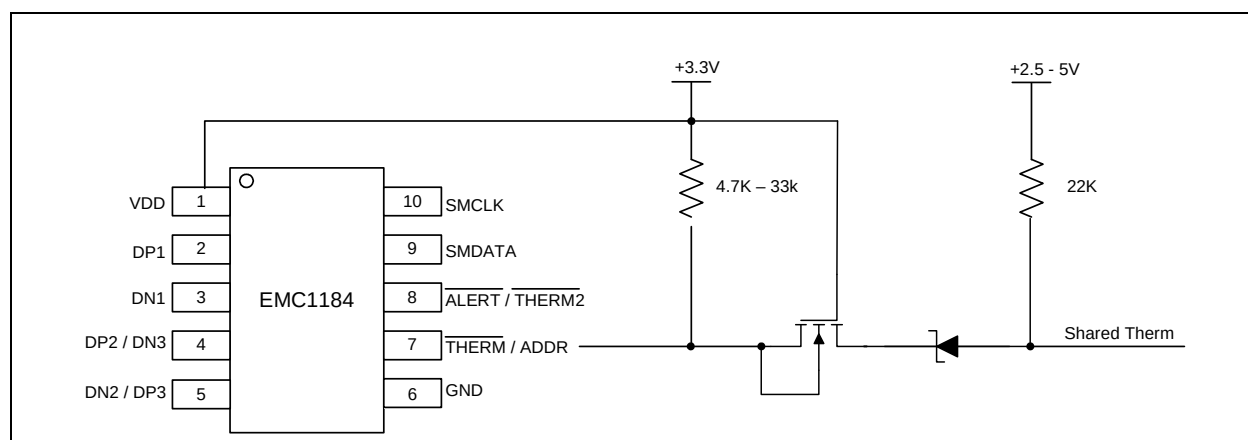
Figure 4.4 Isolating the \overline{\text{THERM}} pin
