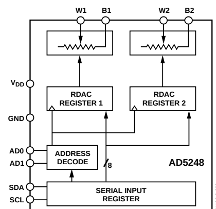
Figure 2. AD5248
