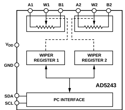
Figure 1. AD5243
