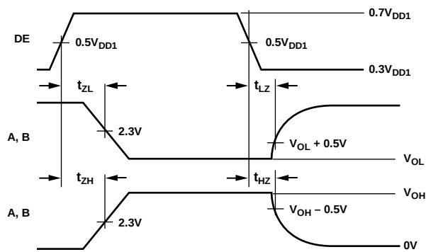
Figure 24. Driver Enable/Disable Timing
