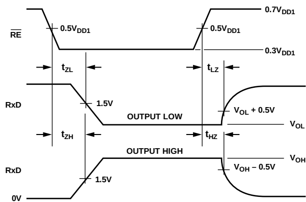
Figure 25. Receiver Enable/Disable Timing
