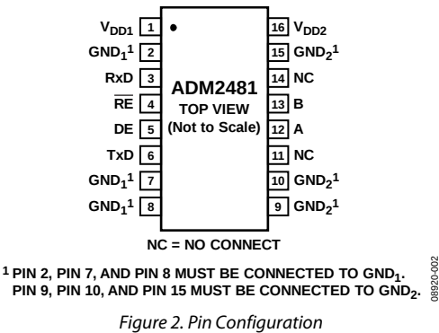
Figure 2. Pin Configuration
