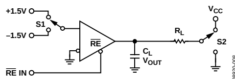
Figure 21. Receiver Enable/Disable
