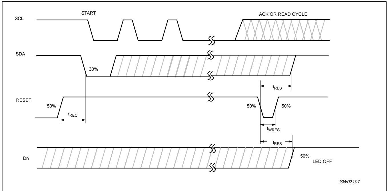
Figure 19. Reset timing
