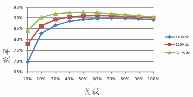
RSD-150D-5
