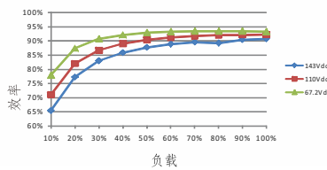
RSD-150D-12
