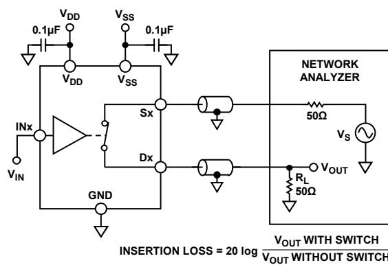
Figure 29. Bandwidth
