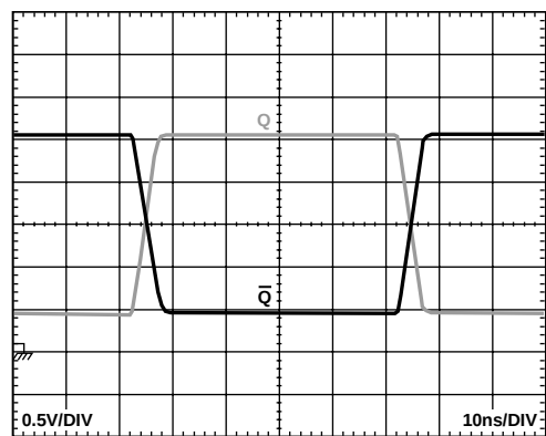
Figure 9. 1 MHz Output Voltage Waveform, V_{CC} = 2.5\text{ V}
