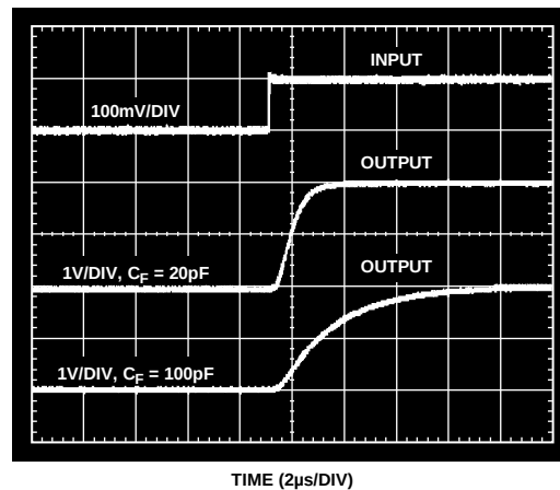
Figure 13. Rise Time
