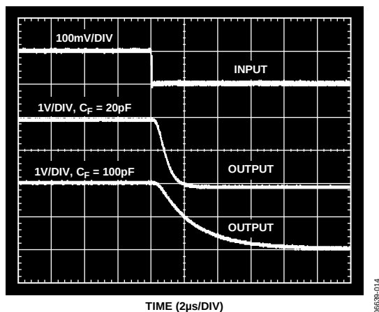
Figure 12. Fall Time
