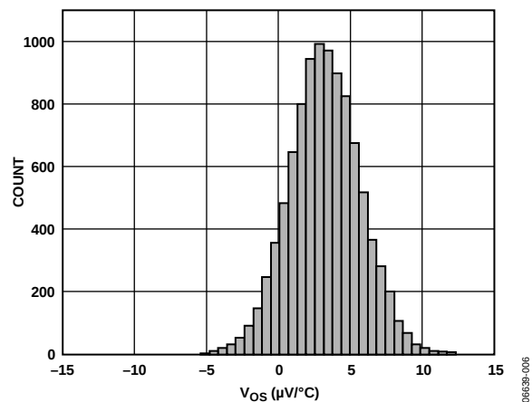
Figure 22. Offset Drift Distribution ( \mu\text{V}/^\circ\text{C} ) (Temperature Range = -40^\circ\text{C} to +125^\circ\text{C} )
