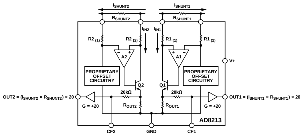
Figure 25. Simplified Schematic
