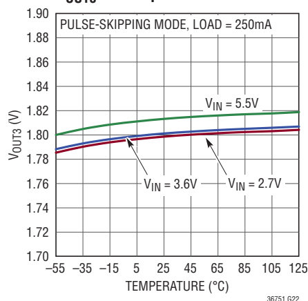
500mA Buck Regulators, V_{OUT3} vs Temperature
