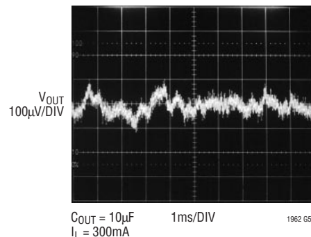
LT1962-5 10Hz to 100kHz Output Noise ( C_{BYP} = 1000pF )
