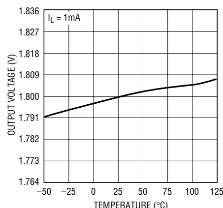
LT1962-1.8 Output Voltage
