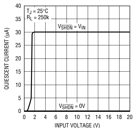
LT1962 Quiescent Current
