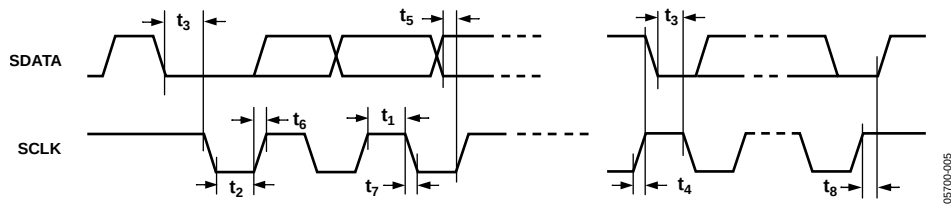
Figure 5. I²C Timing
