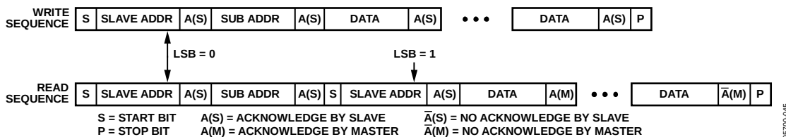
Figure 50. Read and Write Sequence
