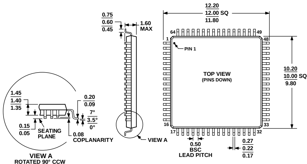
Figure 58. 64-Lead Low Profile Quad Flat Package [LQFP] 10 mm x 10 mm Body (ST-64-2) Dimensions shown in millimeters
