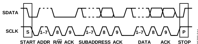
Figure 49. Bus Data Transfer
