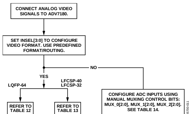
Figure 12. Signal Routing Options
