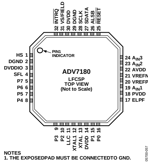
Figure 9. 32-Lead LFCSP Pin Configuration
