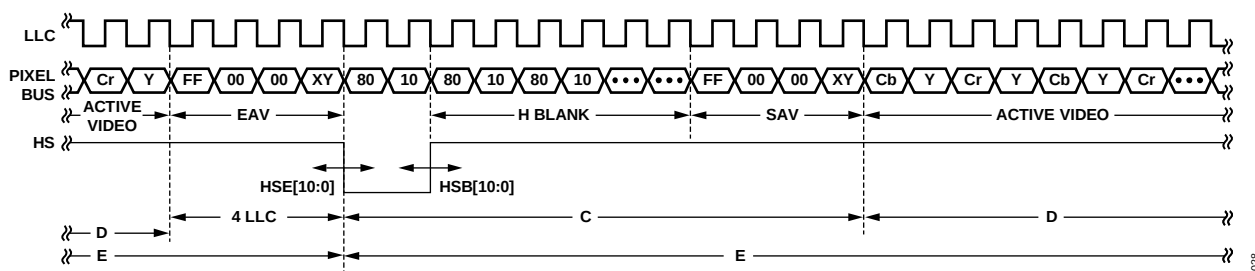
Figure 33. HS Timing
