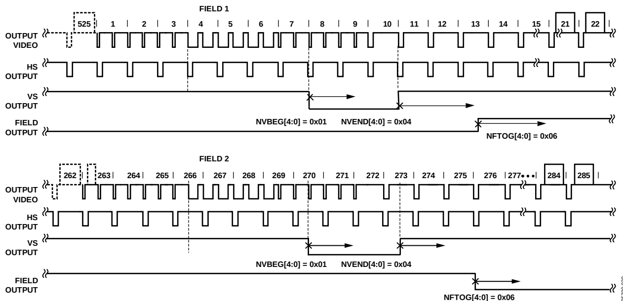
Figure 35. NTSC Typical VSYNC/FIELD Positions Using the Register Writes in Table 64
