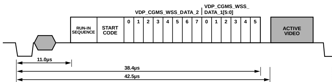
Figure 44. WSS Waveform
