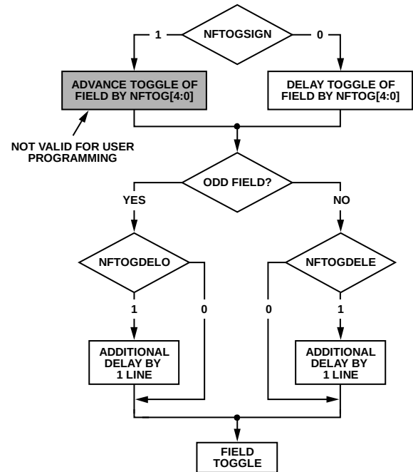
Figure 38. NTSC FIELD Toggle
