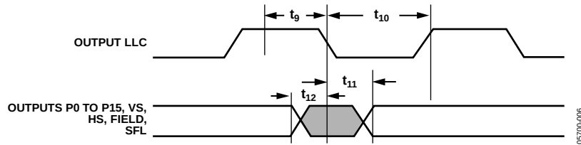
Figure 6. Pixel Port and Control Output Timing
