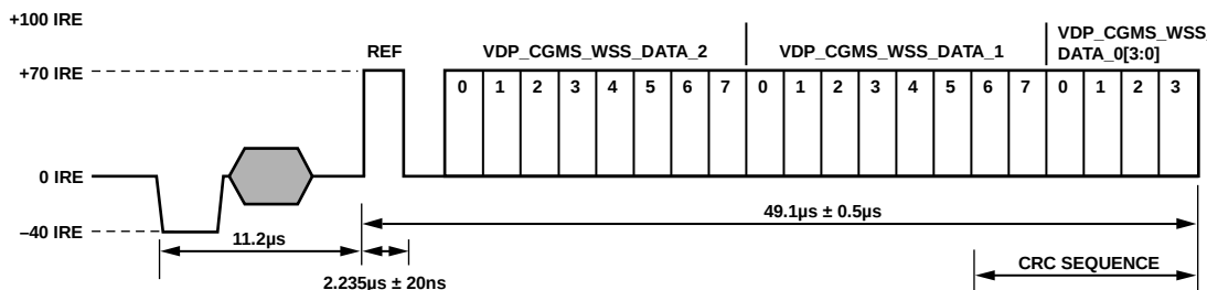
Figure 45. CGMS Waveform
