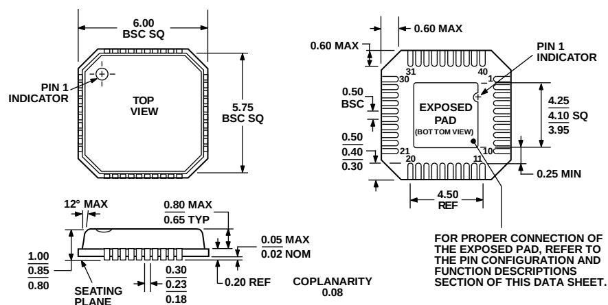
Figure 57. 40-Lead Lead Frame Chip Scale Package [LFCSP_VQ] 6 mm x 6 mm Body, Very Thin Quad (CP-40-1) Dimensions shown in millimeters
