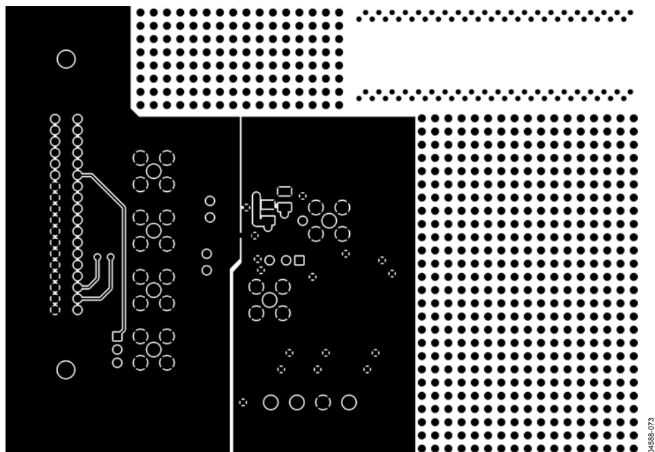
Figure 57. Solder-Side Artwork
