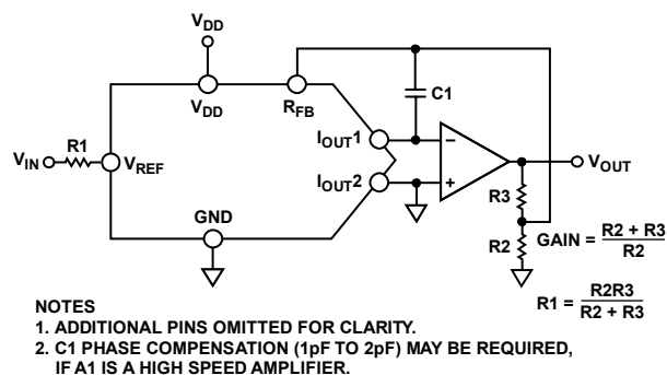
Figure 42. Increasing Gain of Current Output DAC
