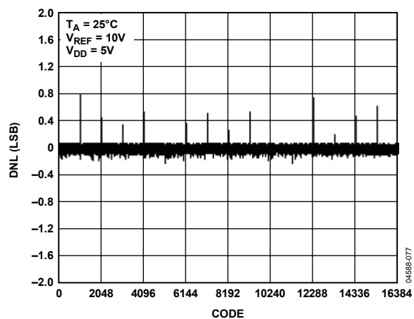
Figure 9. DNL vs. Code (14-Bit DAC)
