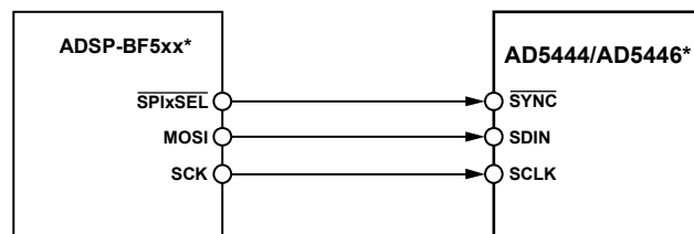
Figure 48. ADSP-BF5xx to AD5444/AD5446 Interface
