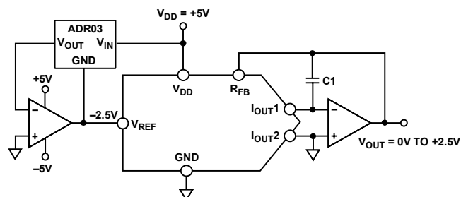
Figure 41. Positive Voltage Output with Minimum Components
