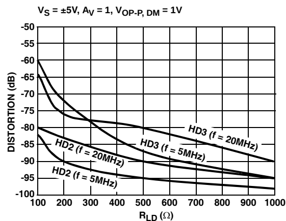
FIGURE 14. HARMONIC DISTORTION vs R_{LD}
