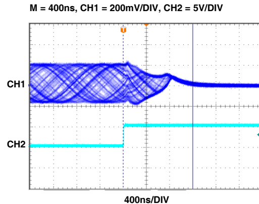
FIGURE 20. DISABLED RESPONSE
