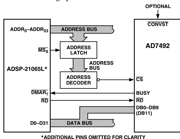
Figure 20. Interfacing to ADSP-21065L
