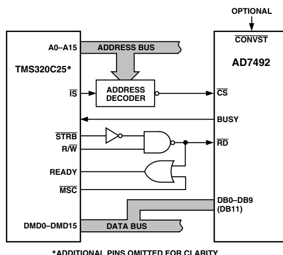
Figure 21. Interfacing to the TMS320C25
