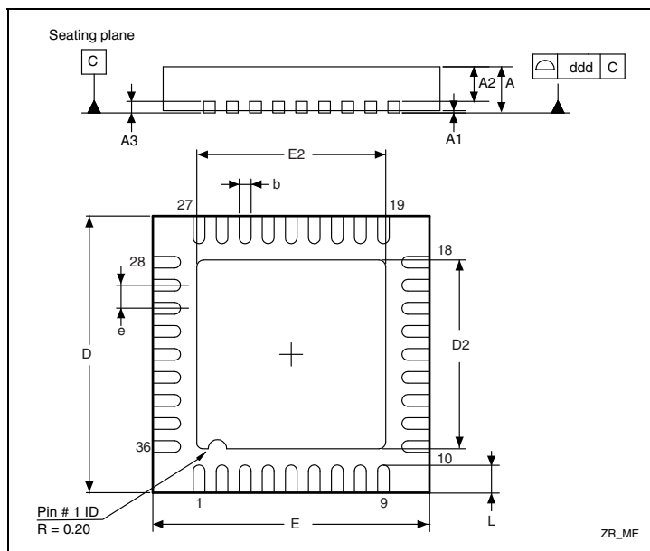
Figure 37. VFQFPN36 6 x 6 mm, 0.5 mm pitch, package outline (1)
