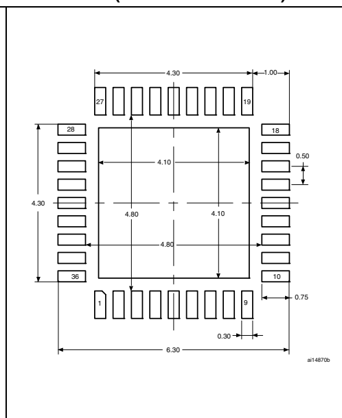
Figure 38. Recommended footprint (dimensions in mm) (1)(2)
