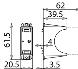
Dimension drawing DG PCB NPE
