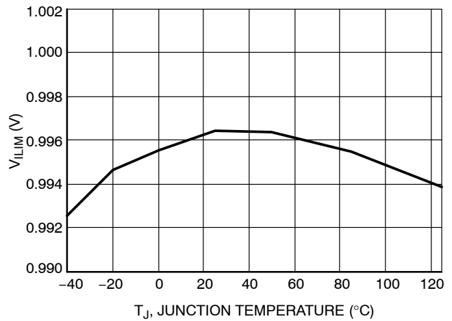
Figure 12. V_{LIM} vs. Junction Temperature
