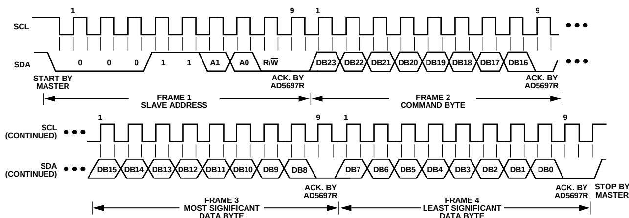
Figure 43. I 2 C Write Operation
