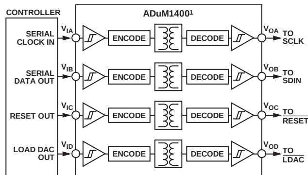
Figure 51. Isolated Interface
