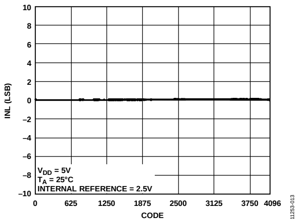
Figure 11. Integral Nonlinearity (INL) vs. Code
