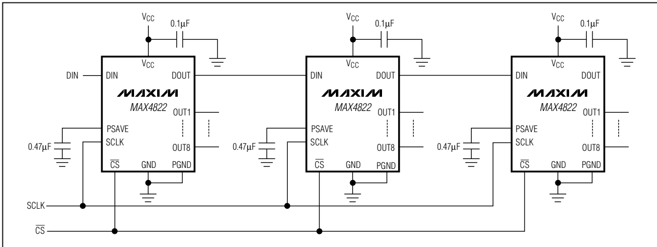
Figure 9. Daisy-Chained MAX4822s with a Capacitor Connected to PSAVE
