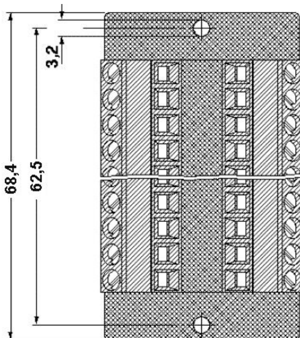
Dimensioned drawing
