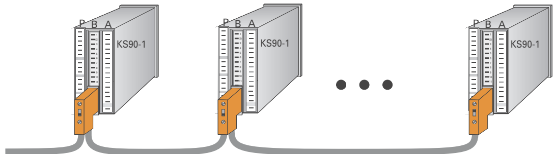
Fig.: 3 Wiring example with sub-D bus adaptor and bus connector
