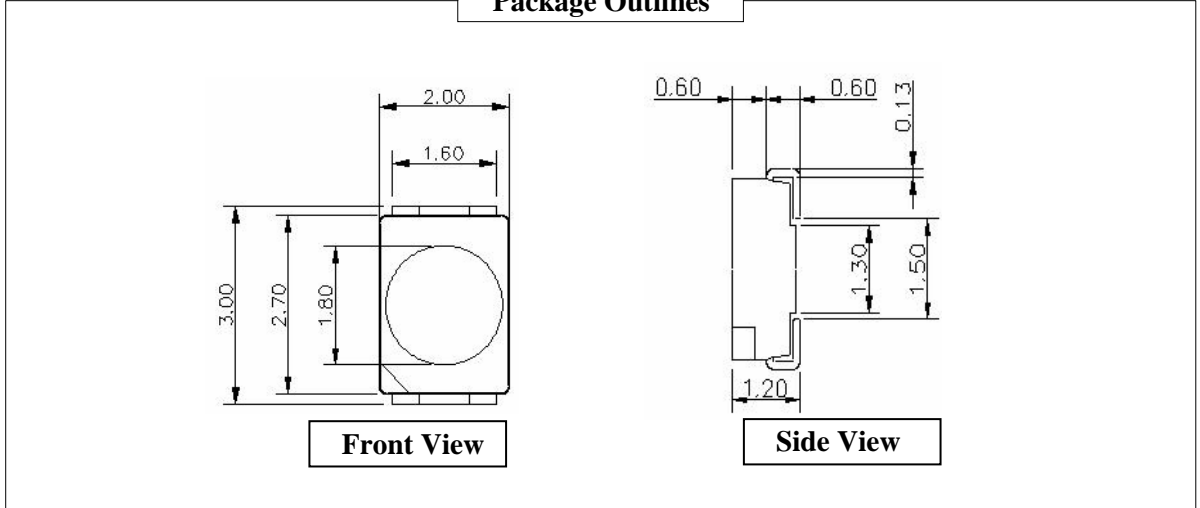
Package Outlines
