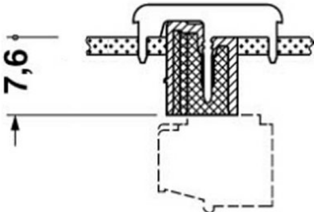
Dimensioned drawing
