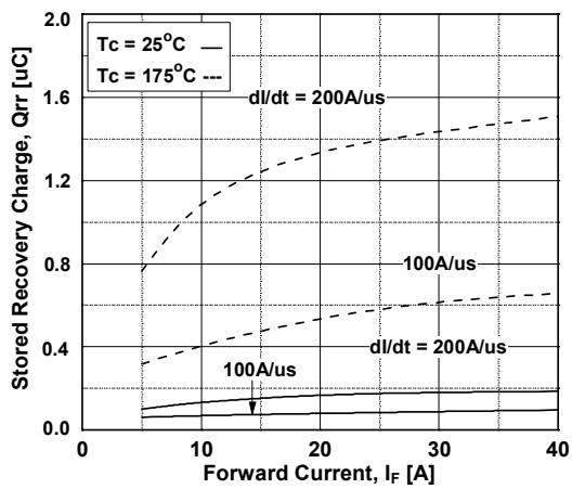
Figure 23. Stored Charge
