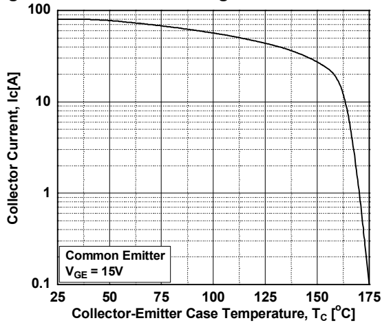
Figure 19. Current Derating
