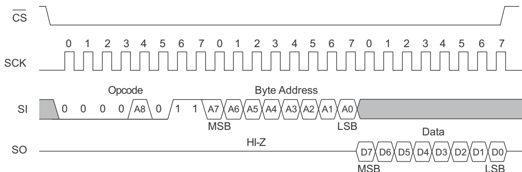
Figure 12. Memory Read
