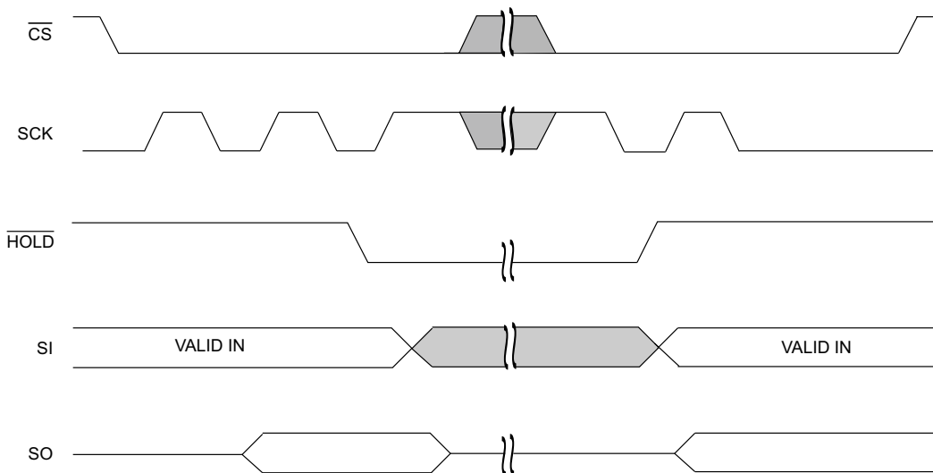
Figure 13. HOLD Operation [2]
