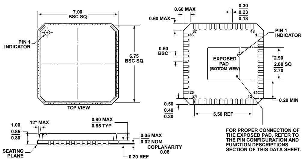
Figure 33. 48-Lead Lead Frame Chip Scale Package [LFCSP_VQ] 7 mm × 7 mm Body, Very Thin Quad CP-48-6
